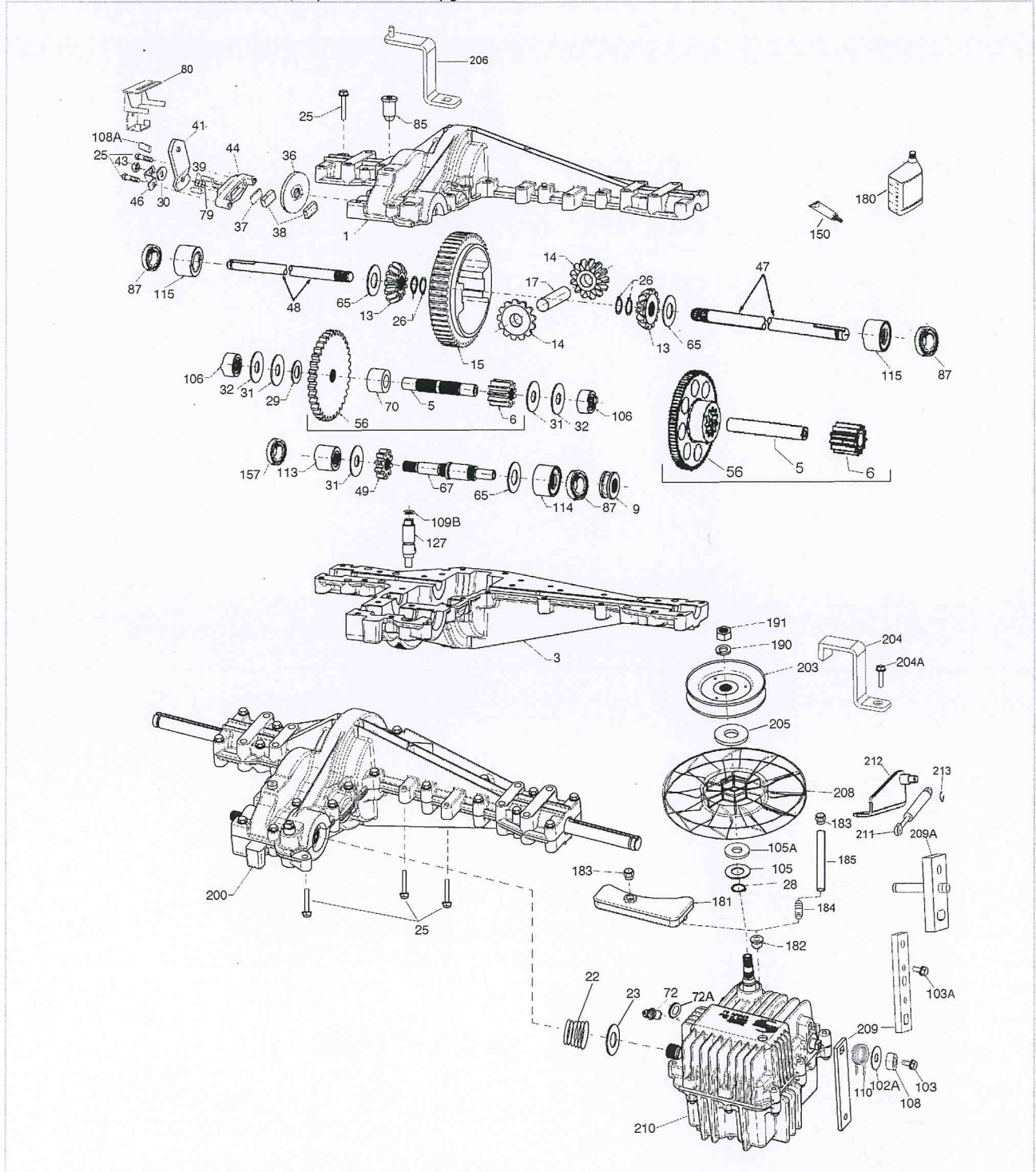
lth2000 2000-2000-006A / Hydro Transaxle pg 1
